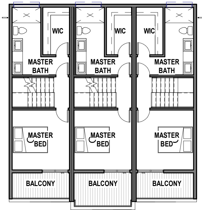
1 LEVEL 3 PLAN #1 : 3/32" = 1'-0"
