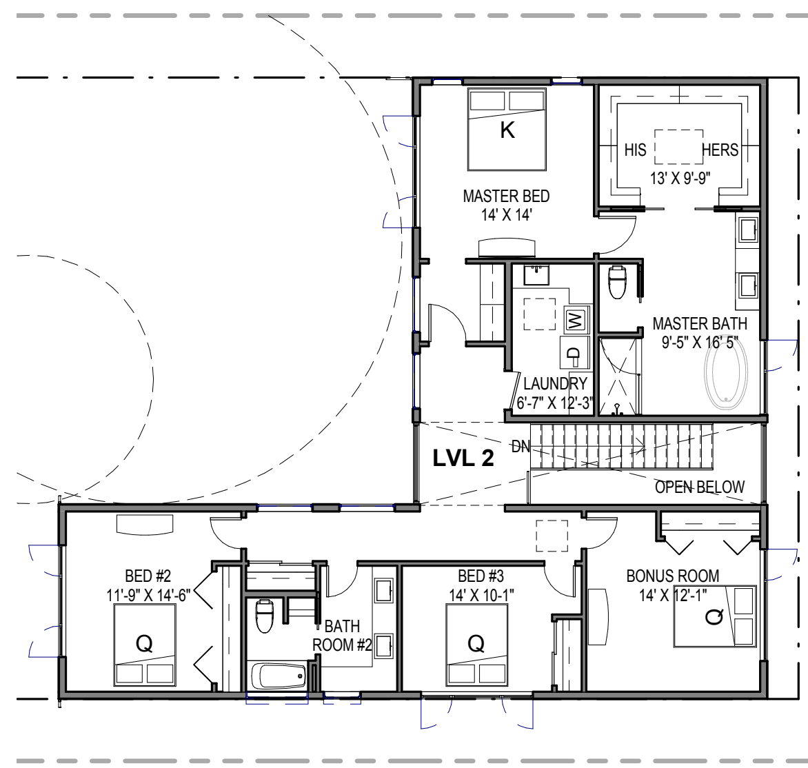
2 LEVEL 2 PLAN : 3/32" = 1'-0"
