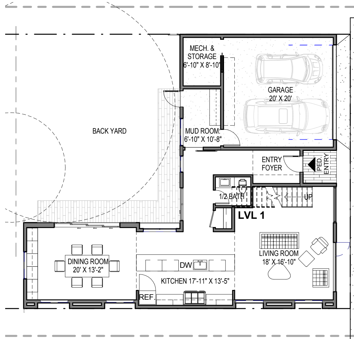
1 LEVEL 1 PLAN : 3/32" = 1'-0"
