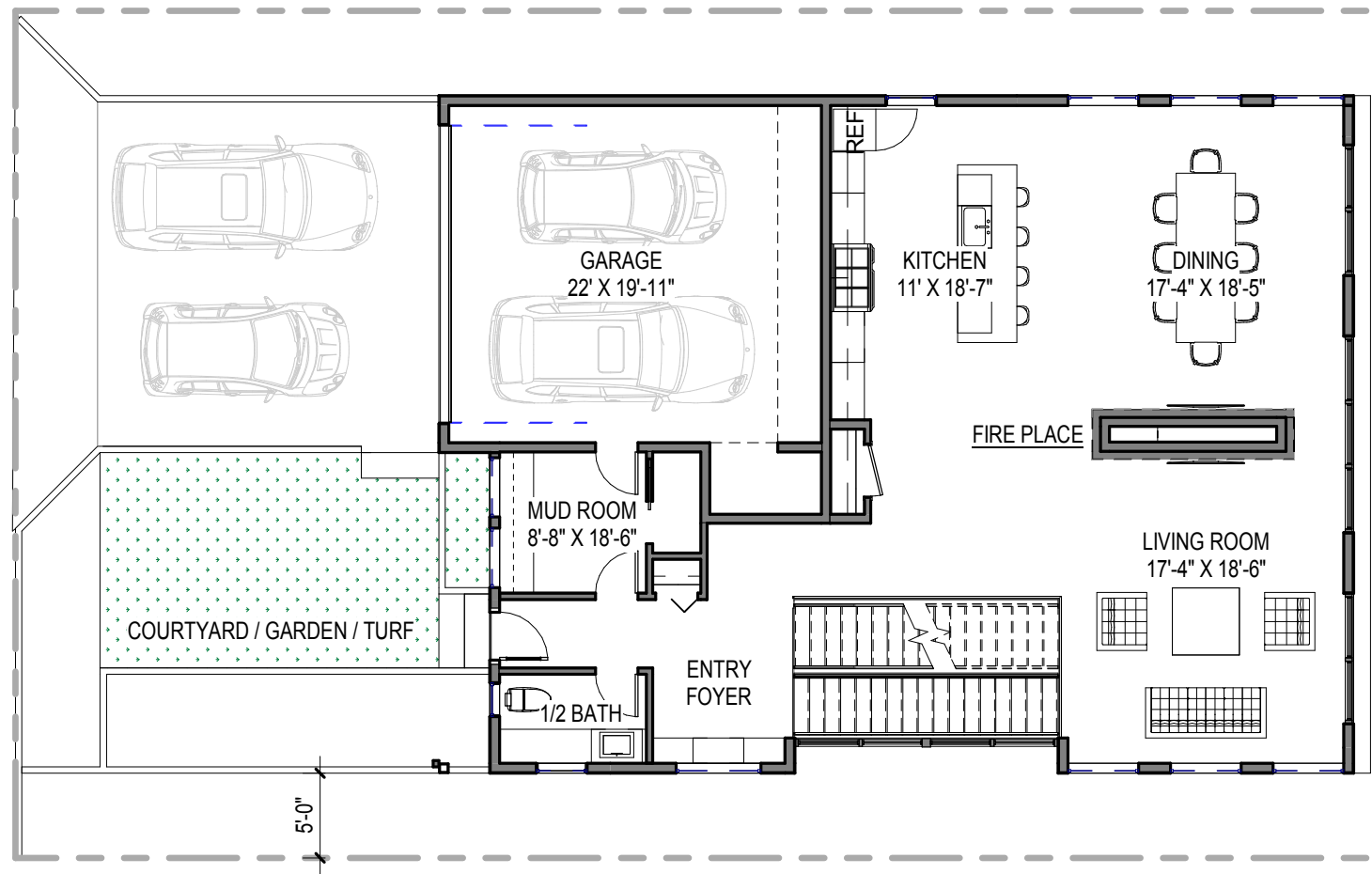
2 LEVEL 1 PRESENTATION : 3/32" = 1'-0"
