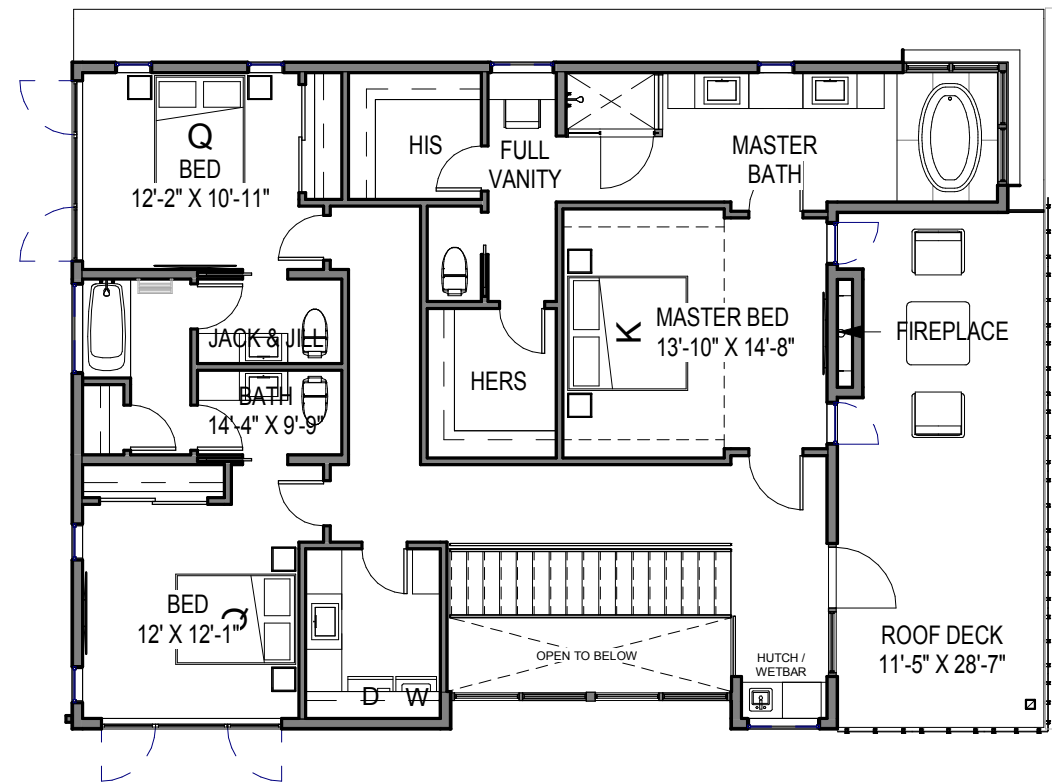
3 LEVEL 2 PRESENTATION : 3/32" = 1'-0"
