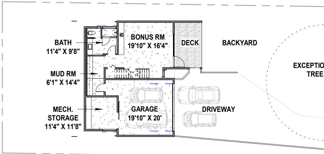
1 LEVEL 0 PLAN : 1" = 20'-0"
